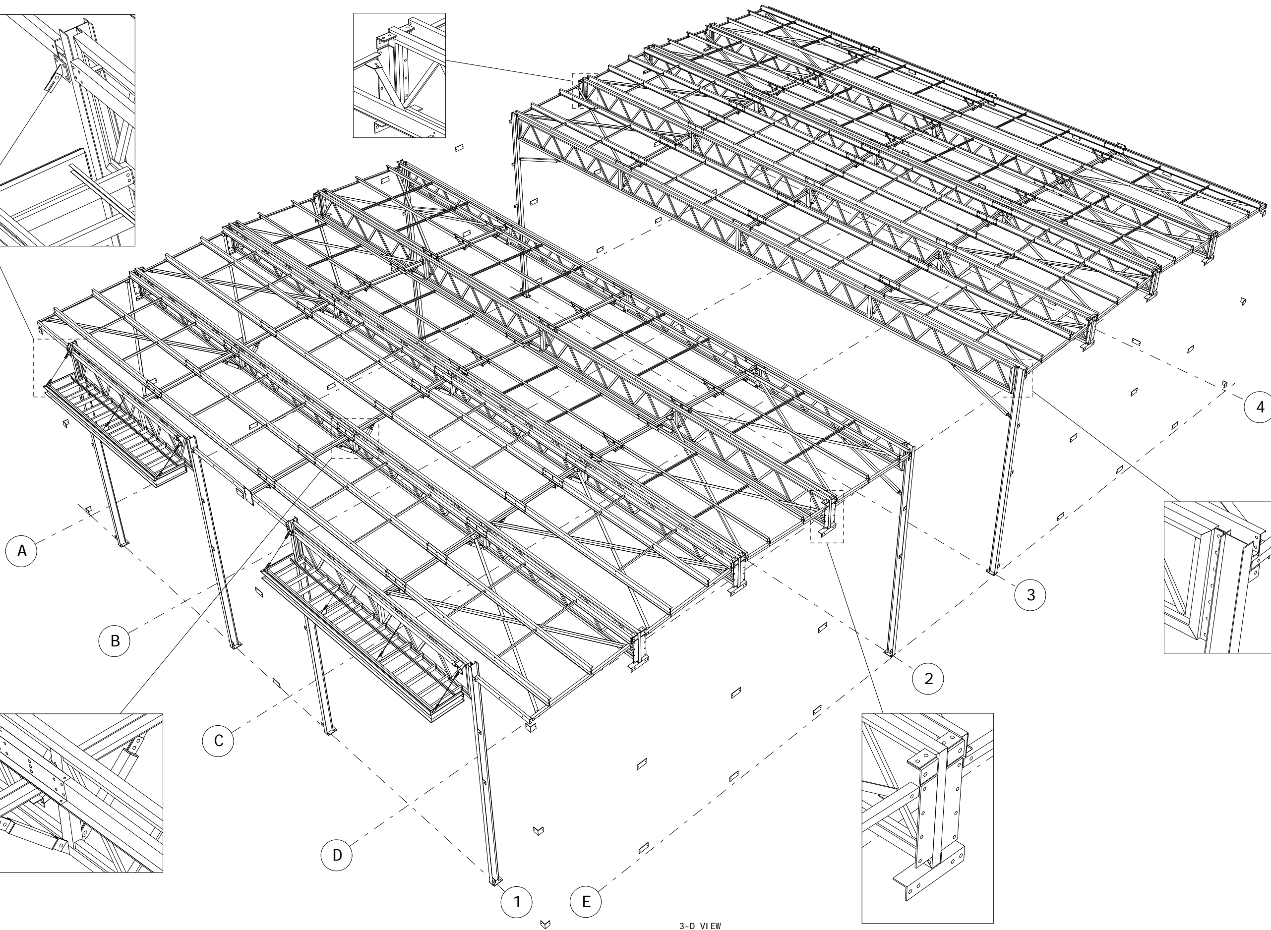
3-D VIEW
